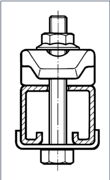
Arrangement A Pass-through bolt with holding bracket L_{min} = a + b + 37 \text{ [mm]}
