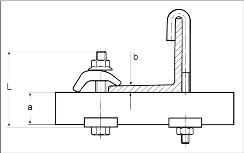
Arrangement A Pass-through bolt with holding bracket L_{min} = a + b + 37 \text{ [mm]}
